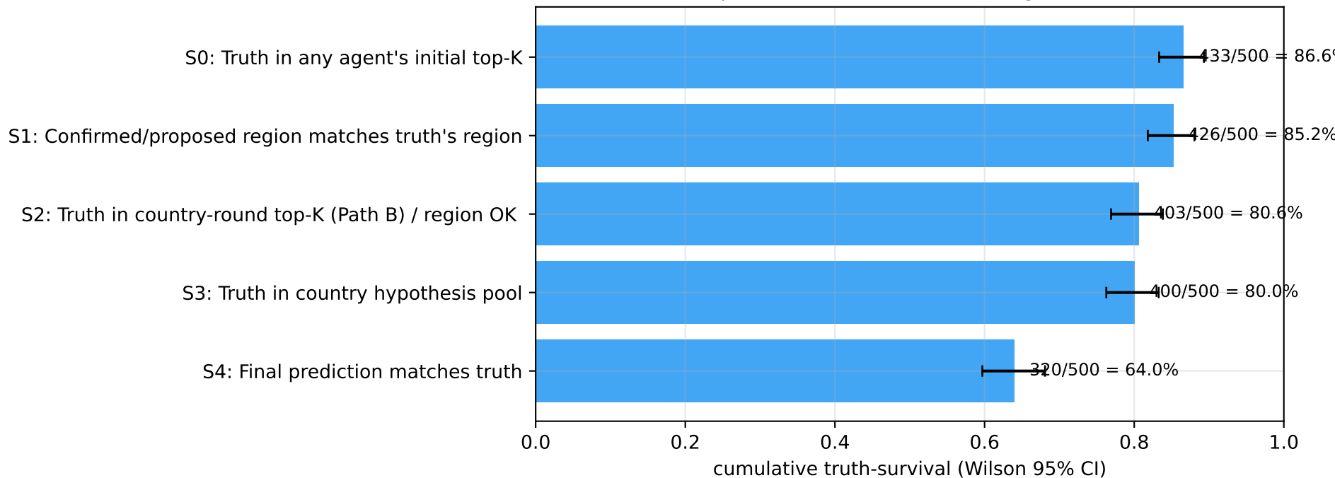
Pipeline funnel, where truth gets lost
